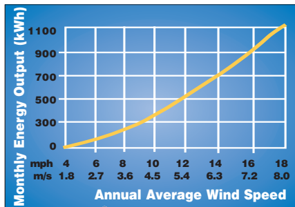
Energy Curve
