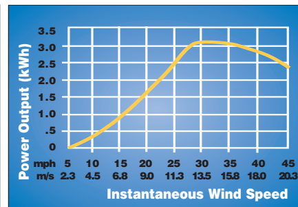
Power Curve
